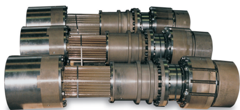
Telescopic quick disengaging spindles.
